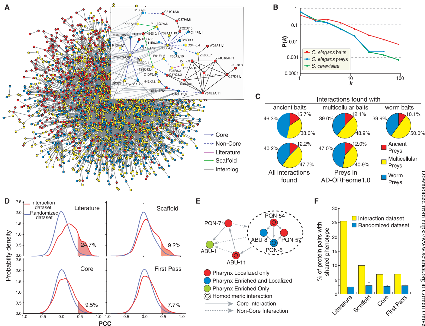
Fig. 2. Analysis of the WI5 network. (A) Nodes (representing proteins) are colored according to their phylogenetic class: ancient (red), multicellular (yellow), and worm (blue). Edges represent protein-protein interactions. The inset highlights a small part of the network. (B) The proportion of proteins, P(k) , with different numbers of interacting partners, k , is shown for C. elegans proteins used as baits or preys and for S. cerevisiae proteins. (C) The pie charts show the proportion of interacting preys found in Y2H screens that fall into each phylogenetic class. Also shown is the distribution of all preys found and all preys searched in the AD-ORFeome1.0 library. (D) Overlap with transcriptome (see text) (18), Pearson correlation coefficients (PCCs) were calculated and graphed for each pair of proteins in the interaction data sets and their corresponding randomized data sets. The red area to the right corresponds to interactions that show a significant relationship to expression profiling data ( P < 0.05 ). (E) Interactions between proteins in Topomap mountain 29 (18). The dash-circled proteins belong to the same paralogous family (sharing more than 80% homology) and are thus collapsed into one set of interactions. (F) Proportion of interaction pairs where both genes are embryonic lethal ( P < 10^{-7} ).
