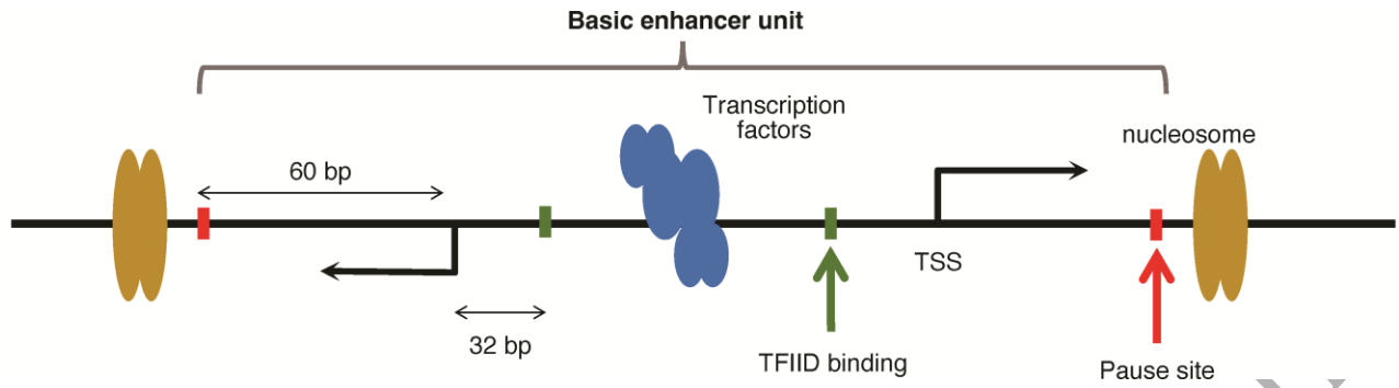
Fig. 1 The architecture of an enhancer unit. The divergent transcription marks the active enhancer and its core components and boundary. Core promoter motifs are located between ~32bp upstream of the TSS (TFIID binding) and ~60bp downstream of TSS (pause sites for RNA polymerase).
