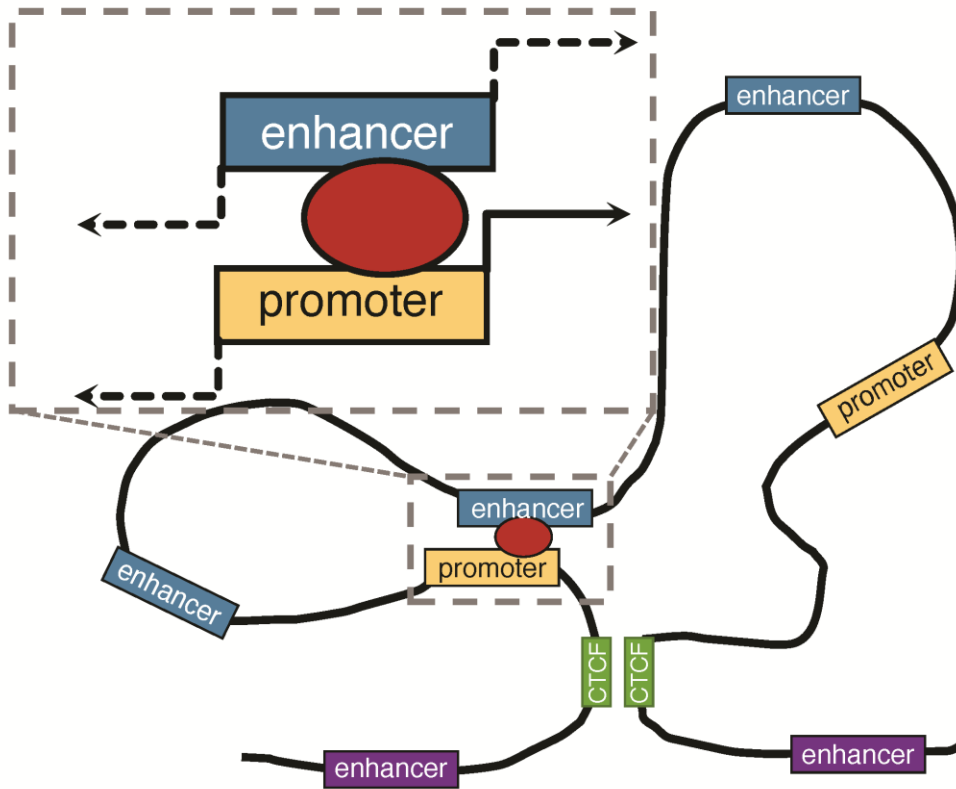
Fig. 2 Illustration of promoter-enhancer interactions within TAD. Across the genome, architectural proteins such as CTCF define TADs to facilitate interaction between elements inside them. CTCF interaction is usually more stable, while interaction between enhancers and promoters are more dynamic. The TAD also serves as an insulator such that enhancers and promoters outside the TAD will have minimal chance to interact with those within the TAD. When gene transcription occurs, unstable and low-abundance transcription also occurs at the other side of the promoter, and in both directions of the enhancer. These divergent transcripts mark the active enhancers in the genome as shown in Fig. 1.
