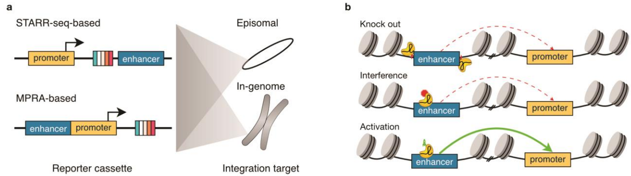
Fig. 3 Illustration of ectopic reporter assays and endogenous perturbation methods for identifying EPIs. (a) Ectopic assays rely on constructing reporter cassettes with promoters and candidate enhancers of interest. Barcodes (BCs) are usually added to the cassettes to make contributions from different elements distinguishable. When integrating the reporter cassettes into plasmids, the following testing is considered episomal, while if the cassettes are integrated into chromosomes, the testing is considered in-genome. (b) The overview of three types of endogenous perturbation methods (CRISPR-based). For interference-based methods, the red octagon represents the fused repressor. For activation-based methods, the green rocket represents the fused activator.
